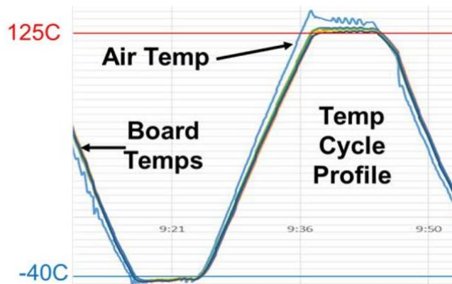
Figure 2. Actual controlled ramp rate, single chamber one hour -40 to 125C BLR temperature cycle profile with thermocouples affixed to the PCBs and monitoring the air.
