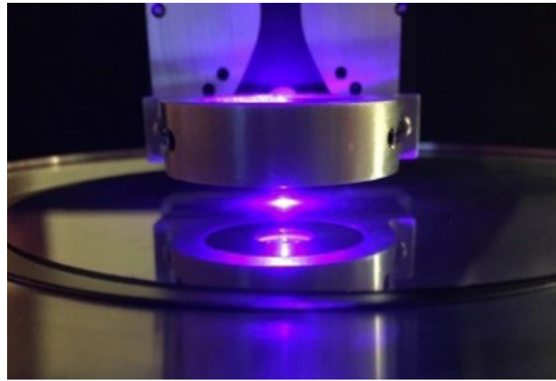
Optical based characterization of diamond materials using transient thermoreflectance (TTR)
